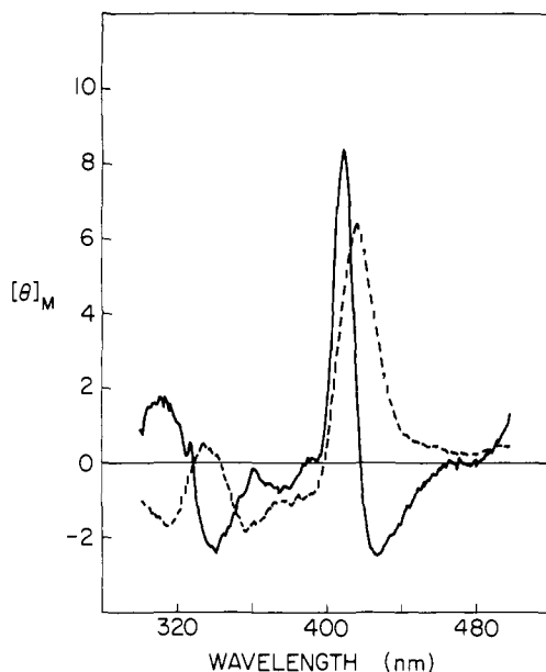
Figure 21. MCD spectra in Soret region of \text{Fe}_2(\beta\text{-FTF4-2,1-NH}) in 0.02 M 1-Melm + 0.01 M pyrazine —; in 0.03 M 1-HIm ---.
