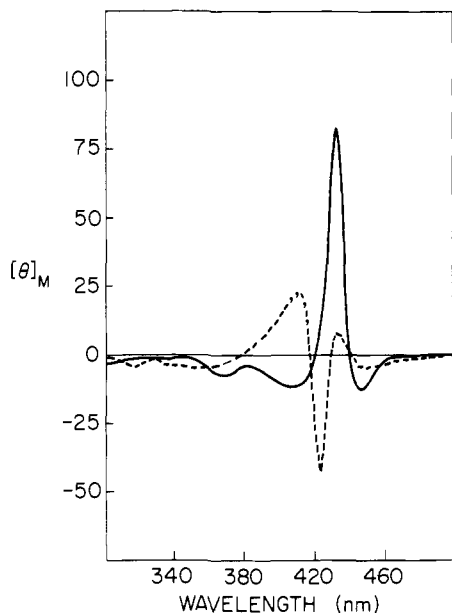
Figure 13. MCD spectra in Soret region of \text{Fe}_2(\text{FTFDU}) in 1-MeIm (excess) —; \text{Fe}_2(\text{ClamDU}) in 1-MeIm (excess) ---.
