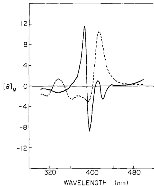
Figure 20. MCD spectra in Soret region of \text{Fe}_2(\beta\text{-FTF4-2,1-NH}) in 0.02 M 1-Melm + CO (1 atm) —; in 0.02 M 1-Melm ---.
