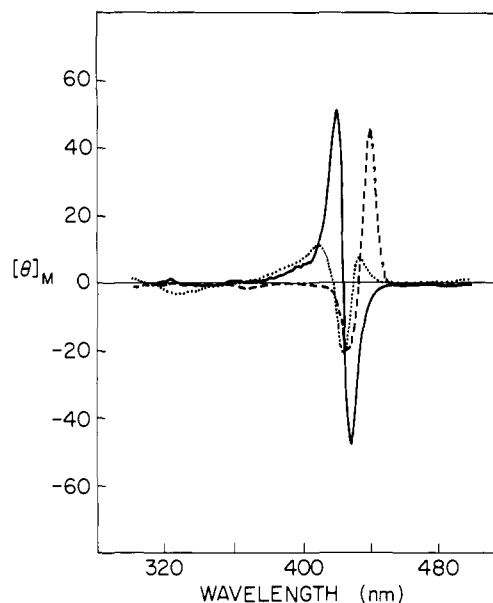
Figure 8. MCD spectra in Soret region of Fe(HmCap) in 0.01 M n -PrNH 2 + CO (1 atm) —; in 0.01 M 1-Melm ---; in 0.01 M n -PrNH 2 ···.
