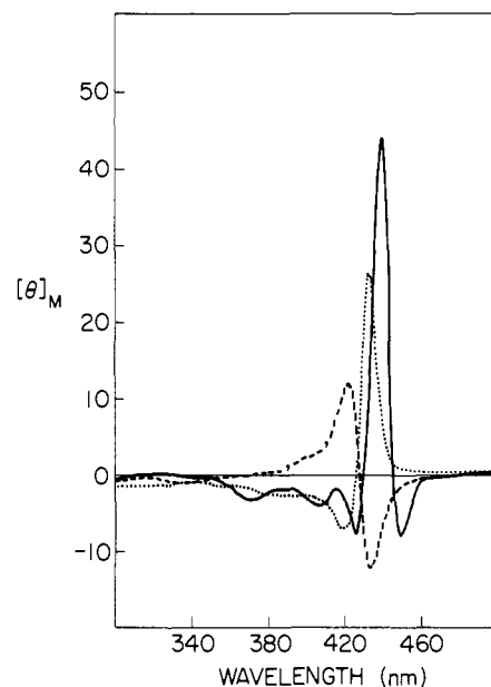
Figure 11. MCD spectra in Soret region of Fe(PocPivP) in 1-MeIm (2.0 M) —; in 1-MeIm (excess) + CO (1 atm) ---; in toluene-THF (1:1) ····.
