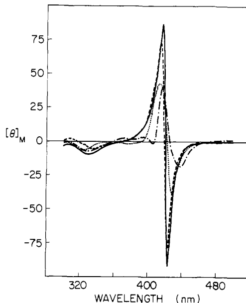
Figure 14. MCD spectra in Soret region of \text{Fe}_2(\text{FTFDU}) in 1-TrIm (excess) + CO (1 atm) —; \text{Fe}_2(\text{ClamDU}) in 1-MeIm (excess) + CO (1 atm) ---; \text{Fe}_2(\text{FTFDU}) in 1-TrIm (excess) + pyrazine (excess) ····; in pyrazine (excess) ···.
