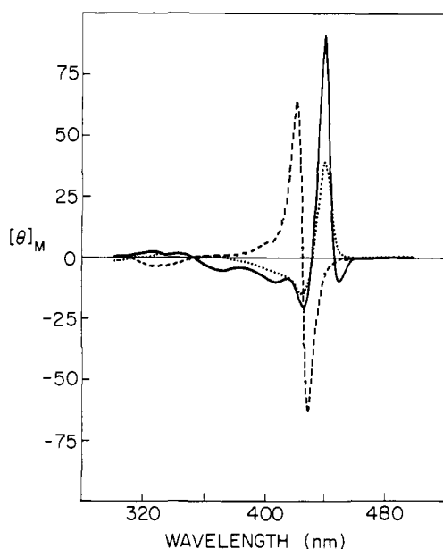
Figure 7. MCD spectra in Soret region of Fe(Cap) in 2 M 1-Melm —; in 1 M n -PrNH 2 + CO (1 atm) ---; in pyridine (excess) ···.
