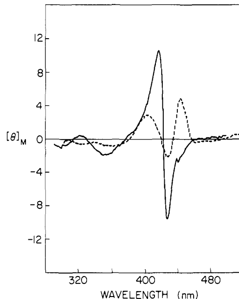
Figure 18. MCD spectra in Soret region of \text{Fe}_2(m\text{-FTF5-3,1-NH}) in 0.1 M 1-MeIm + CO (1 atm) —; in 0.1 M 1-MeIm ---.
