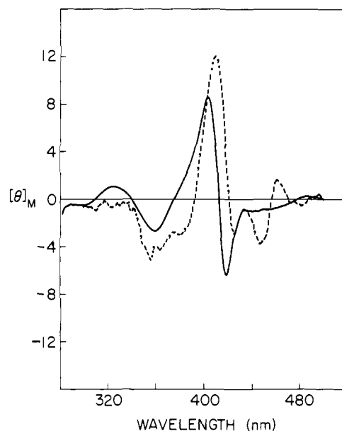
Figure 22. MCD spectra in Soret region of Ni(ADE) —; \text{Fe}_A\text{Ni}_N(\beta\text{-FTF6-3,2-NM3}) ---.
