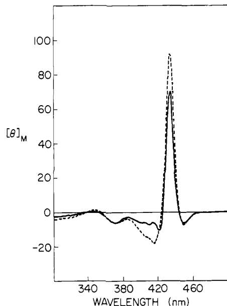
Figure 12. MCD spectra in Soret region of \text{Fe}_2(\text{ClamDU}) in 1-TrIm (excess) —; \text{Fe}_2(\text{FTFDU}) in 1-TrIm (excess) ---.
