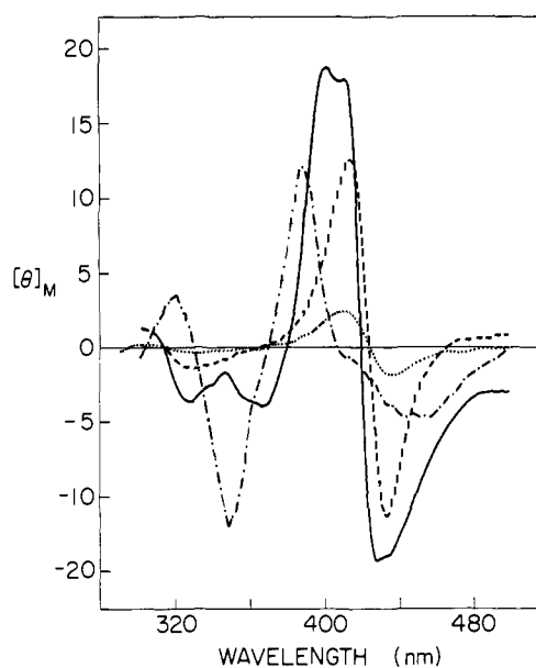
Figure 23. MCD spectra in Soret region of [\text{Fe}(\text{TPP})]_2\text{O} —; \text{Fe}[\text{Piv}_3(4\text{CImP})\text{P}] + \text{O}_2 (1 atm) ---; \text{Fe}_2(\beta\text{-FTF4-2,1-NH}) in 0.4 M 1-Melm + \text{O}_2 (1 atm) ····; \text{Fe}(\text{PocPivP}) in 1-Melm excess + \text{O}_2 (1 atm) - · - ·.
